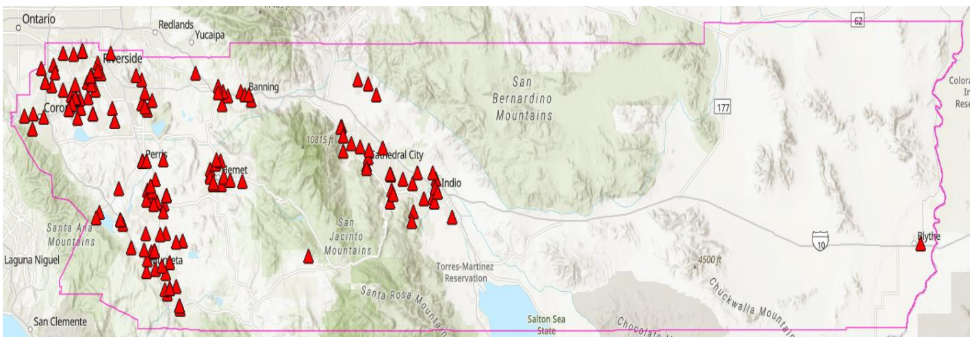
ILI-related EMS response in Riverside County, ePCR distribution map: Week 51
