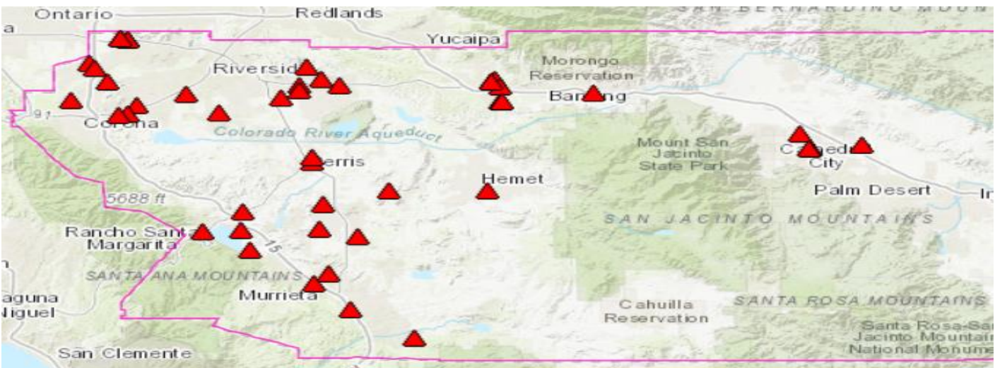
ILI-related EMS response in Riverside County, ePCR distribution map: Week 27
